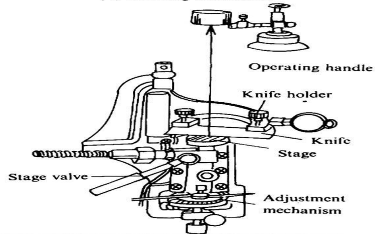
(4) Freezing microtome
