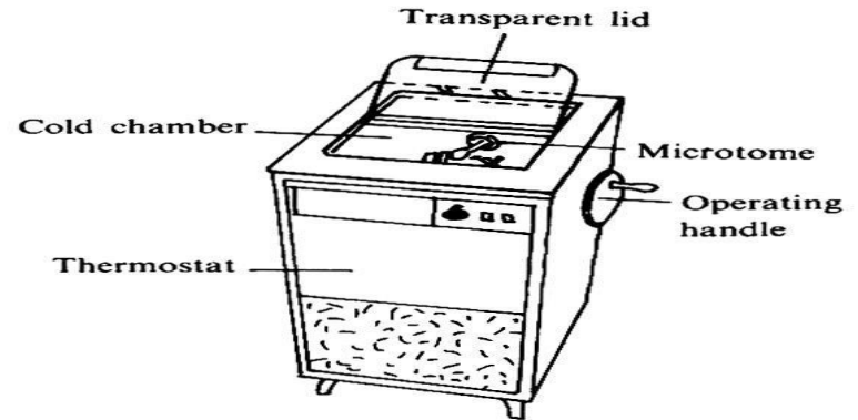
(2) Cryostat
